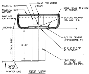
INSULATED BOX SUPPORT
